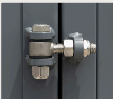
Adjustable stainless-steel hinges ensure door alignment
