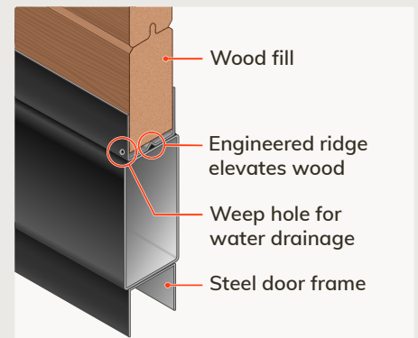
Integrated water drainage protects wood
