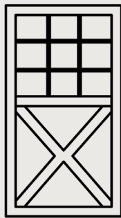
DDF-2 Framed for Glass w/ 9 Lite Mullions, Wood Bottom w/ Crossbucks
